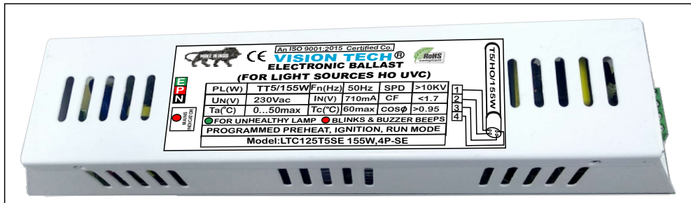
UV5: DIMENSION: L=278mm, W=55mm, H=42mm
